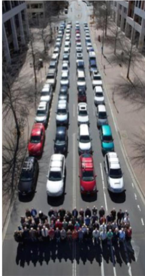
PRIVATE VEHICLE
