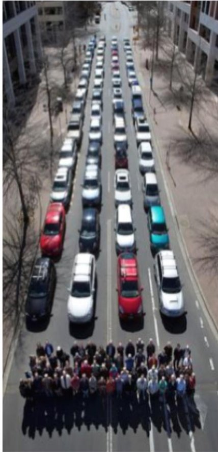
AUTOMATED VEHICLE
